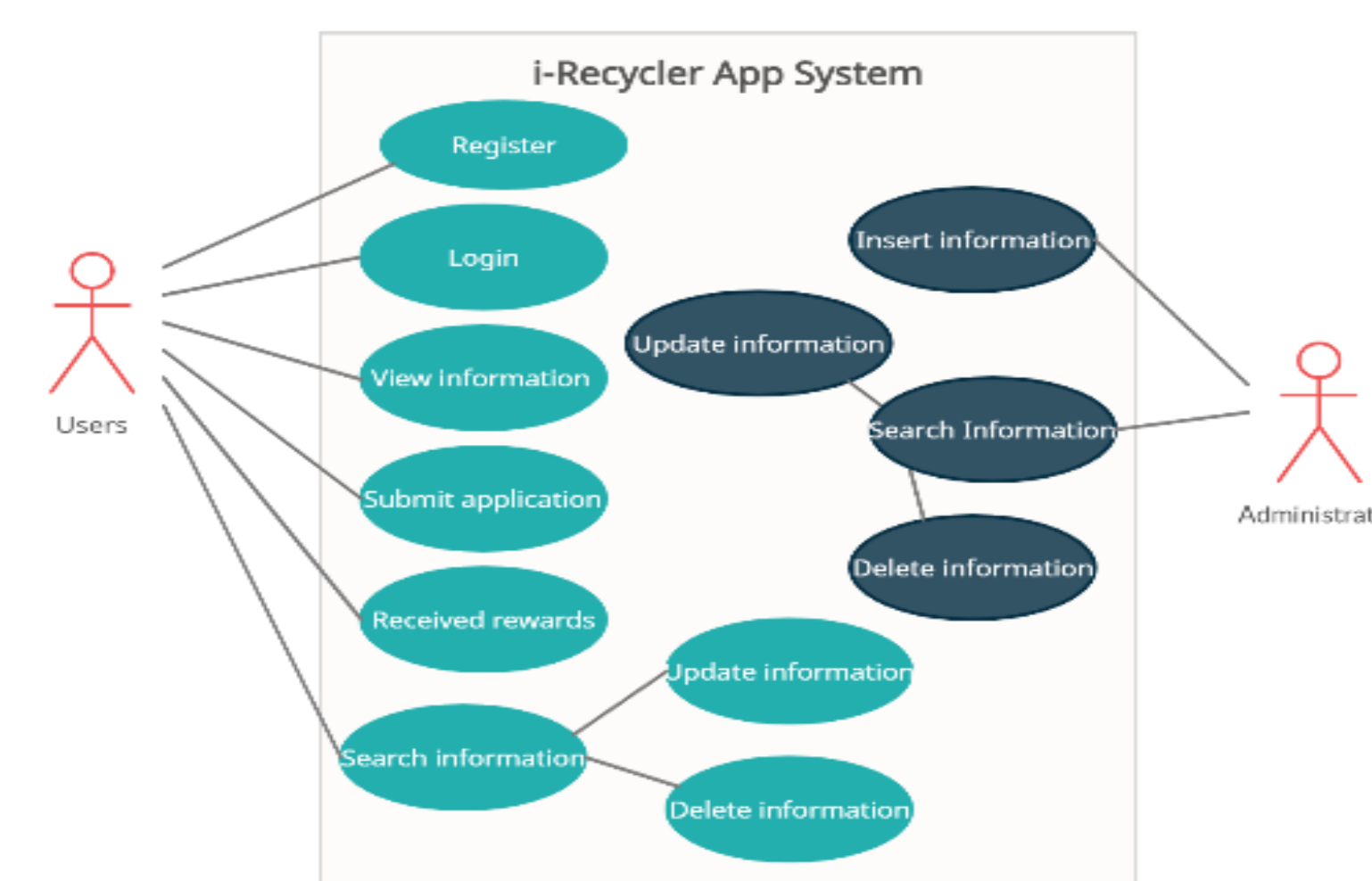
Figure 2: Use Case Diagram of i-Recycler App System
